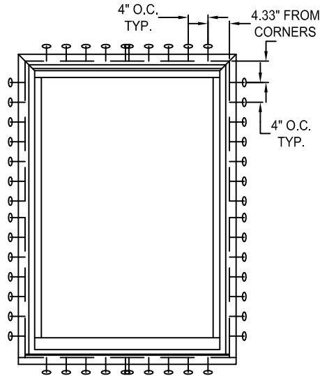
TYPICAL ELEVATION WITH FASTENER SPACING
